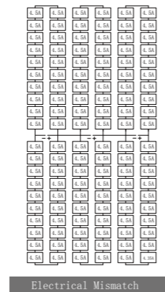
Electrical Mismatch
