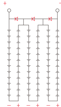
Circuit Diagram
